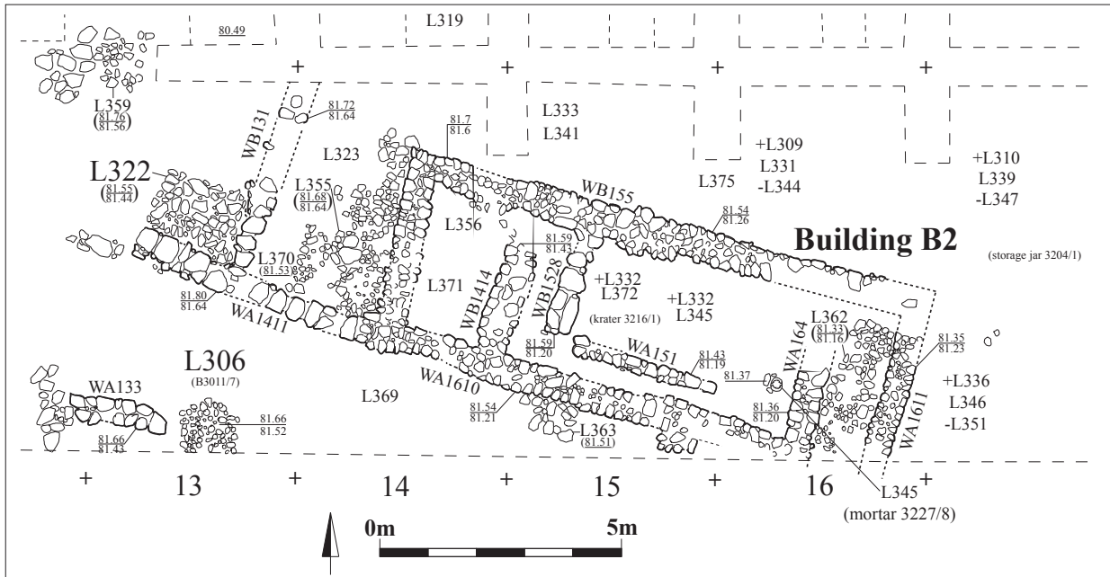
Fig. 2.8. Plan of Building B2.
